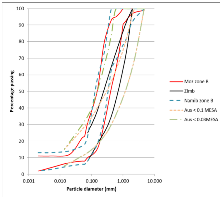
Figure 5-4: Grading envelopes for sands
