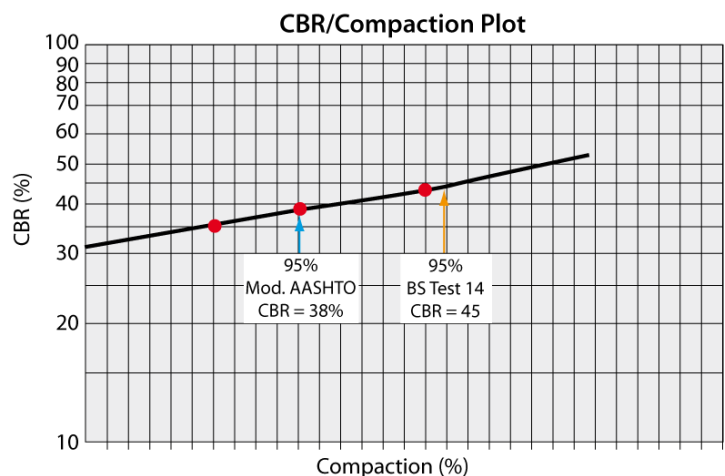
Figure 3-10: CBR/compaction relationship
