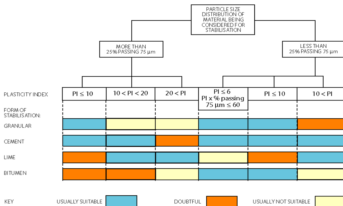
Figure 5-6: Guide to the method of stabilization (Austroads, 1998)
