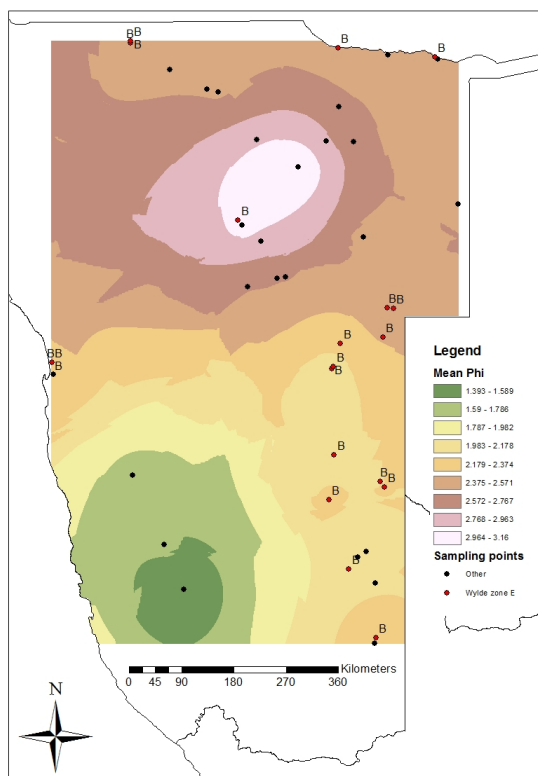
Figure 3-6: Distribution of mean (Phi units) of sands in Namibia
