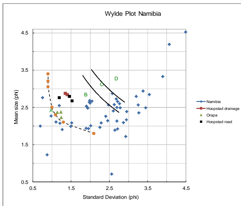
Figure 4-11: Classification of all sands based on grading (Phi units)
