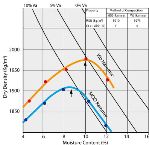
Figure 3-9: Density/voids relationship
