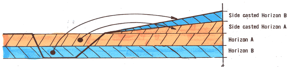
Figure 6.3 – Grader side-casting of in situ material
