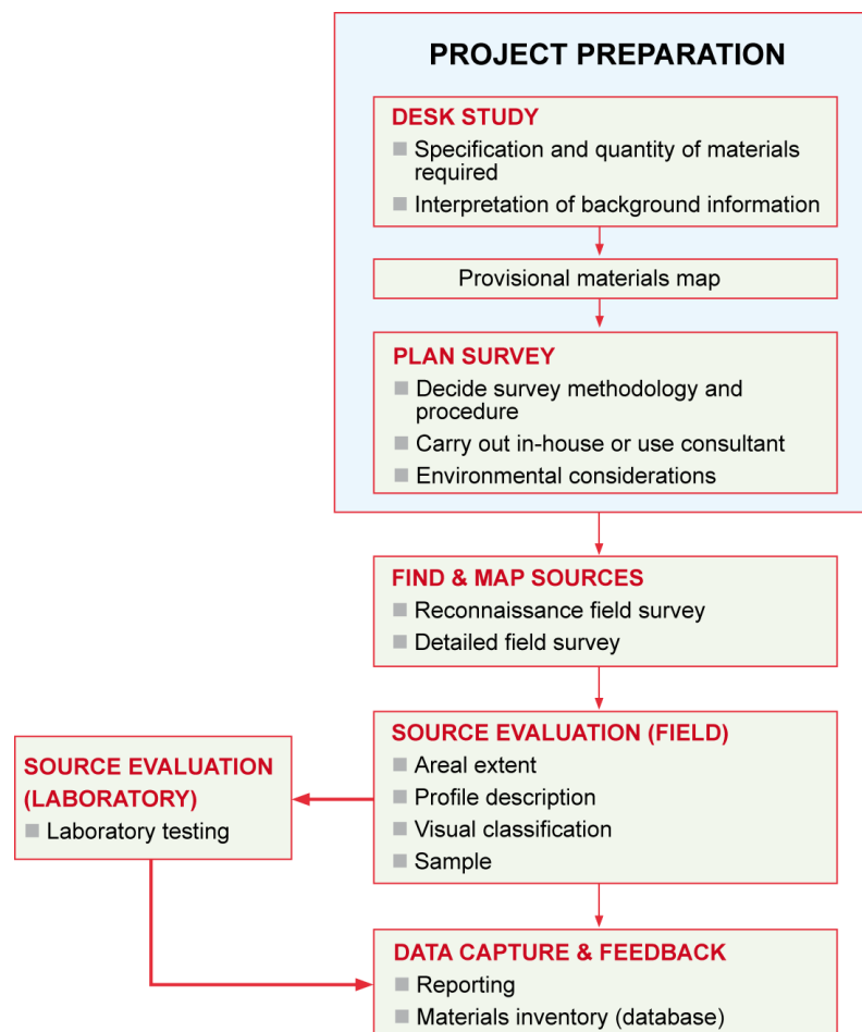
Figure 3-1: Flow diagram stages for sand prospecting
