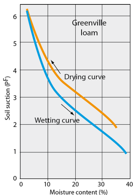
Figure 4-19: Soil suction/moisture content relationship (Wooltorton, 1954)
