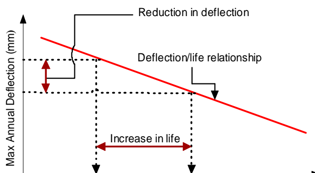
Figure 6.2 – Deflection/life relationship
