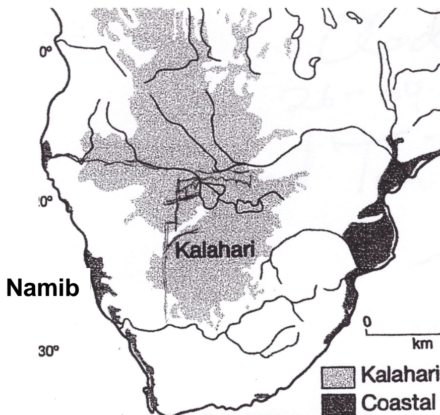
Figure 2-2: Distribution of sands in southern Africa (Cooke, 1964)
