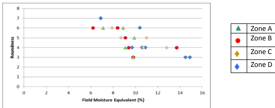
Figure 4-14: Field moisture equivalent versus roundness
